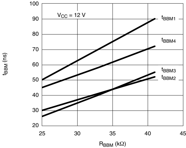
t_{BBM} vs. R_{BBM} , V_{EP} = 0\text{ V} , V_{LX} = 48\text{ V} , BST = 60\text{ V} , V_{INDET} = 4.8\text{ V} , f_{OSC} < 200\text{ kHz}
